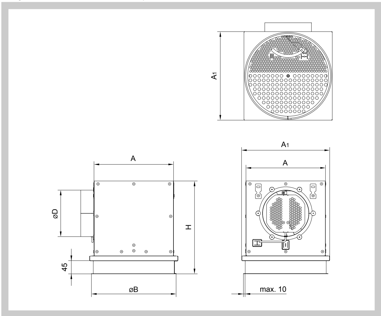
Fig. 4 Horizontal connection, round front plates
