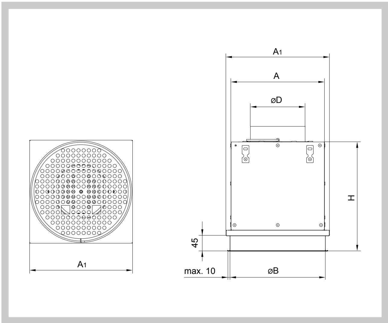
Fig. 6 Vertical connection, round front plates
