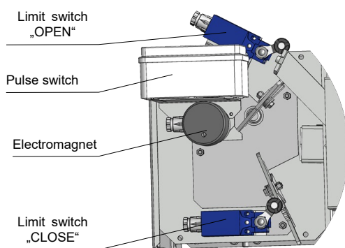
Fig. 11 Design .82, .83 - design with mechanical control, electromagnet (solenoid) and limit switches
