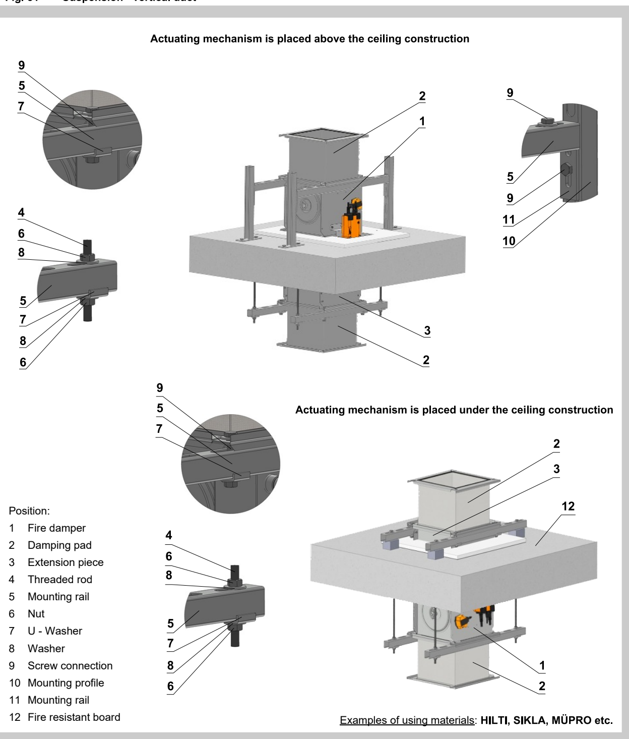
Fig. 51 Suspension - vertical duct
