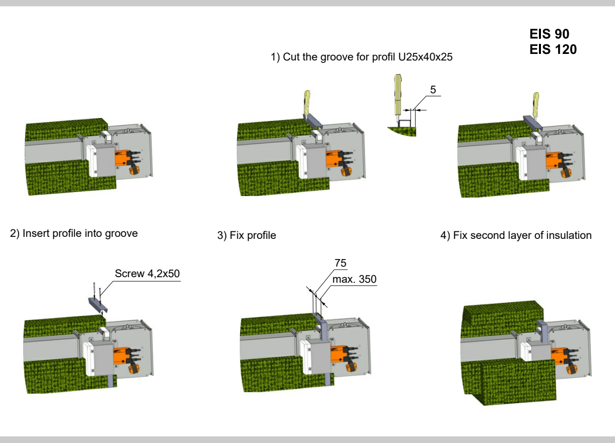
Fig. 48 Installation procedure
