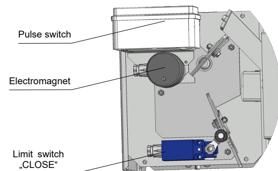
Fig. 9 Design .23, .24 - design with mechanical control, electromagnet (solenoid) and limit switch
