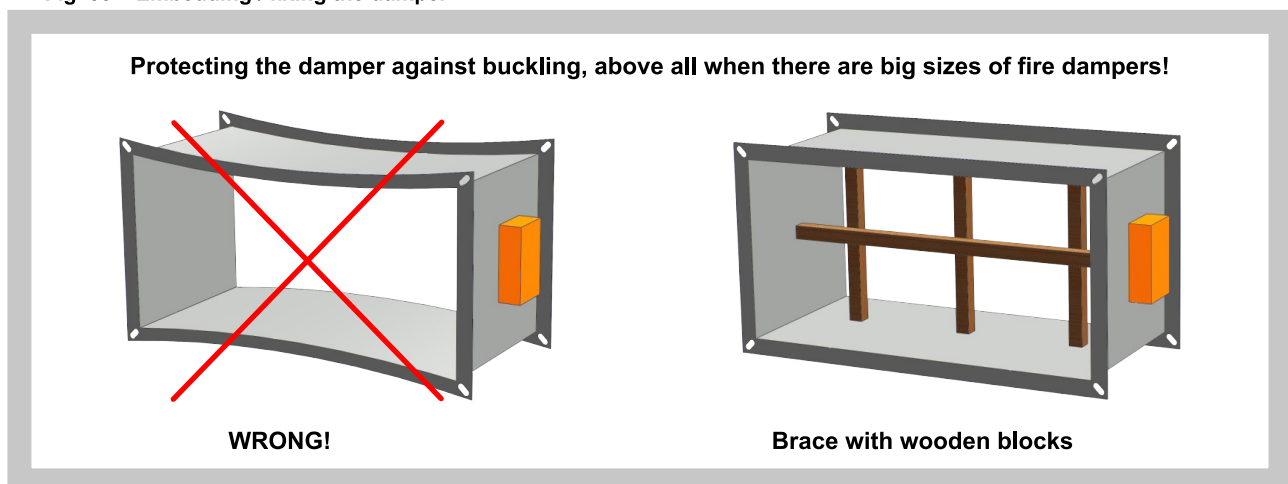
Fig. 53 Embedding / fixing the damper
