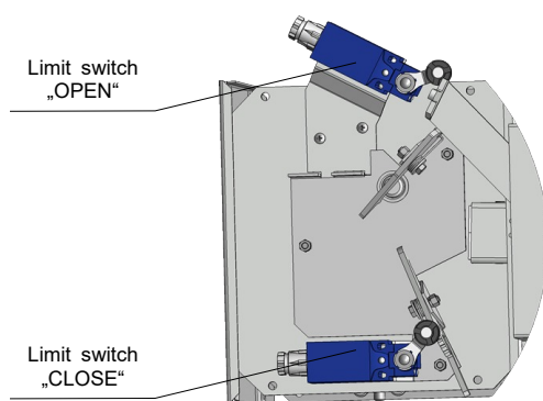
Fig. 10 Design .80 - design with mechanical control and limit switches „OPEN“, „CLOSE“
