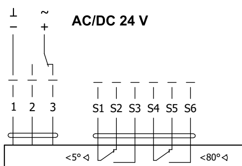
Fig. 10 Actuator BELIMO BEE 24(-ST)
