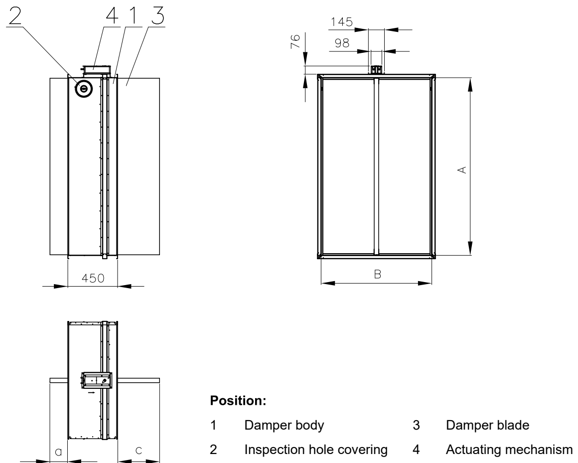
Fig. 3 Single compartment smoke control damper
