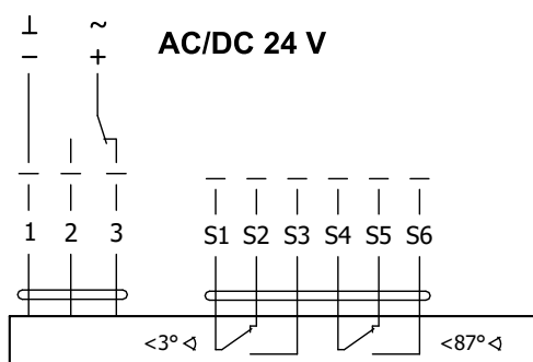
Fig. 12 Actuator BELIMO BE 24-12(-ST)
