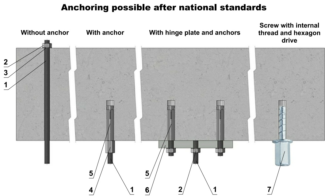
Fig. 7 Mounting to the ceiling wall
