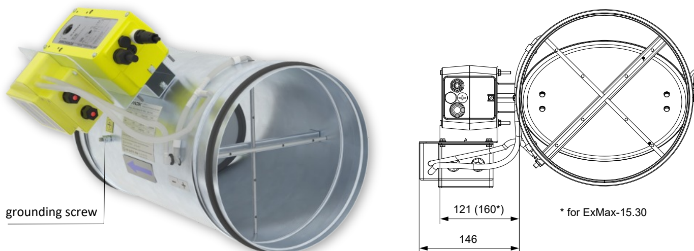
RPM-V with Schischek electrical equipment
