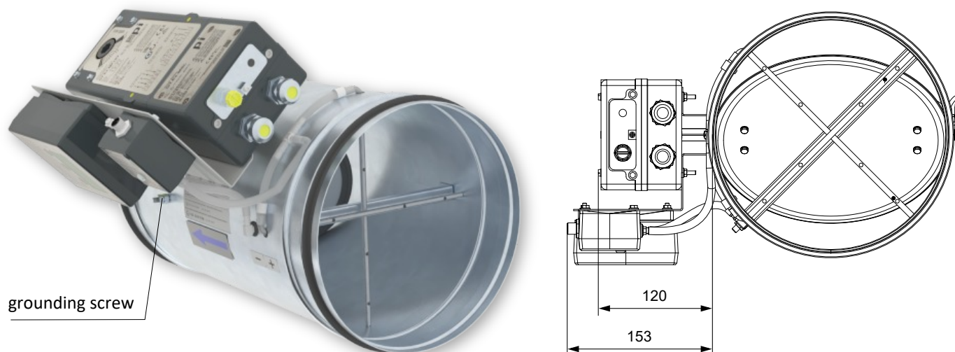
RPM-V with pi safety electrical equipment
