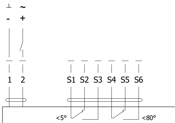
Actuator BELIMO BFN 230, BFN 24
