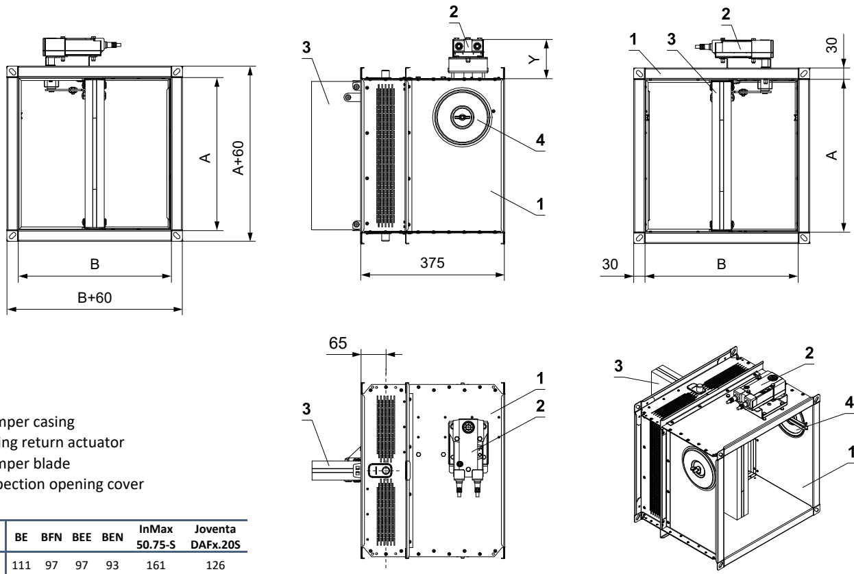
Square MSD - design with spring return actuator and insulation box
