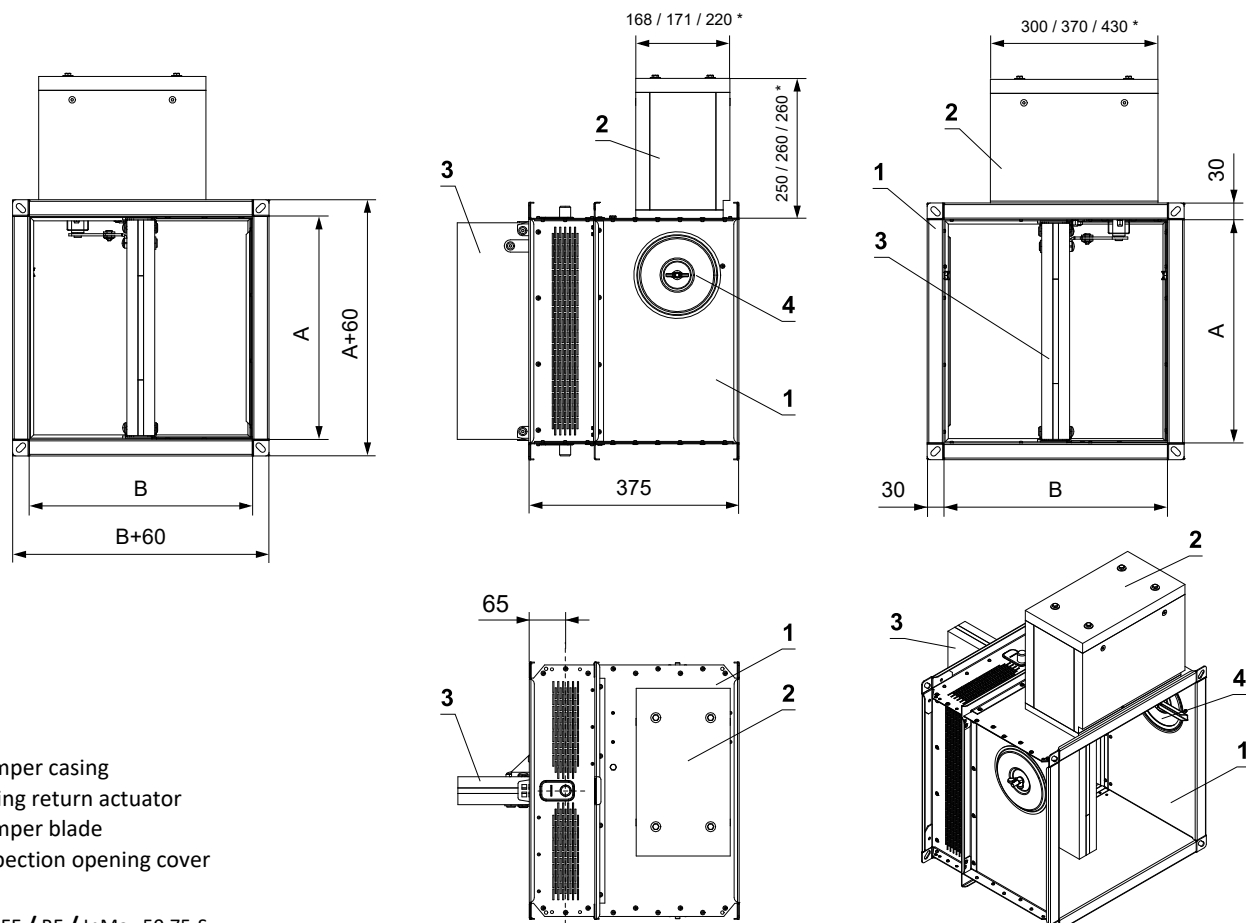
Square MSD - design with spring return actuator and insulation box
