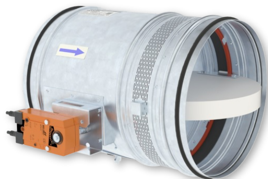
MSD - round
