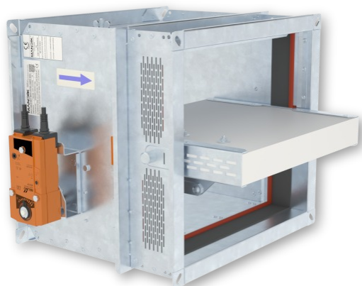
MSD - square
