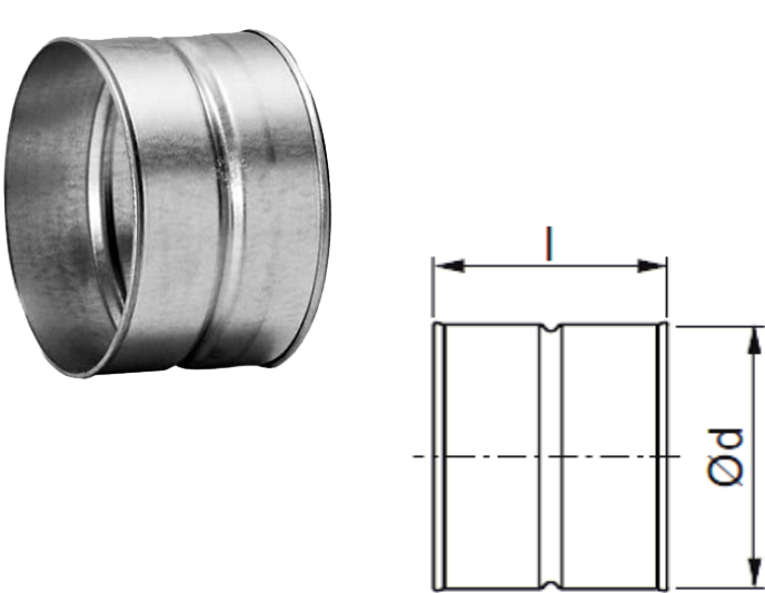
Female coupling
